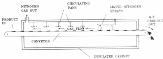
Figure 25 Liquid nitrogen freezer
